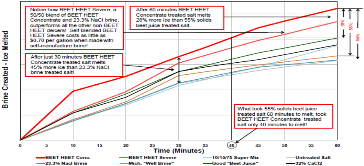
Treated Salt Ice Melt Capacity Test Results @ 15°F Modified SHRP 205.1 Ice Melt Capacity Solids Advanced Laboratories, Inc. Salt Lake City, UT - Margin of Error 3.6%
