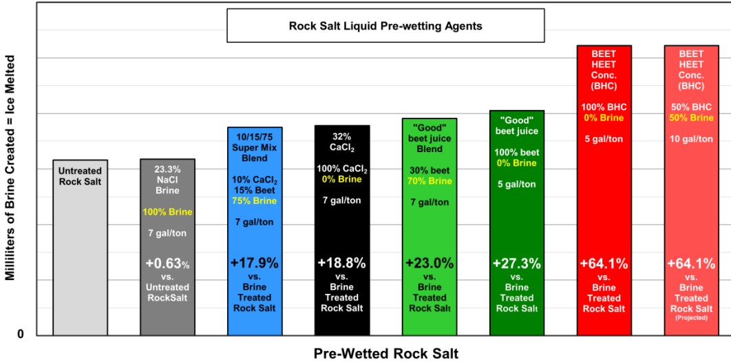
Pre-Wetted Rock Salt - Treated Rock Salt Needed Comparison @ 25°F Based On Modified SHRP H-205.1 Ice Melt Capacity Solids Advanced Laboratories, Inc. Salt Lake City, UT - Margin of Error 3.6%
